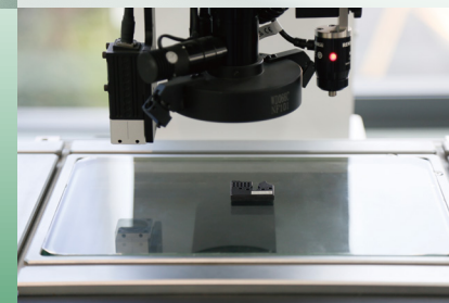
Workpiece Measurement
